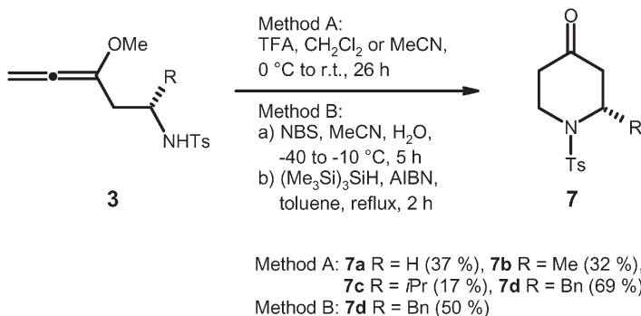
SCHEME 5 Cyclization of unpurified adducts 3 to piperidinones 7
