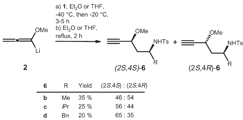
SCHEME 4 Conversion to alkynes 6
